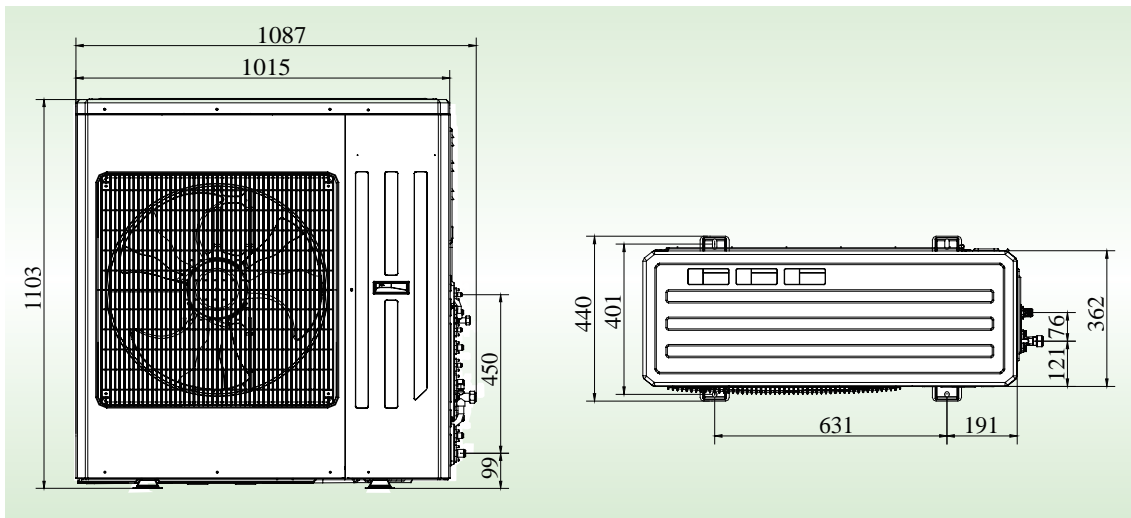
Dimensions for:GWHD(42)NK3AO
